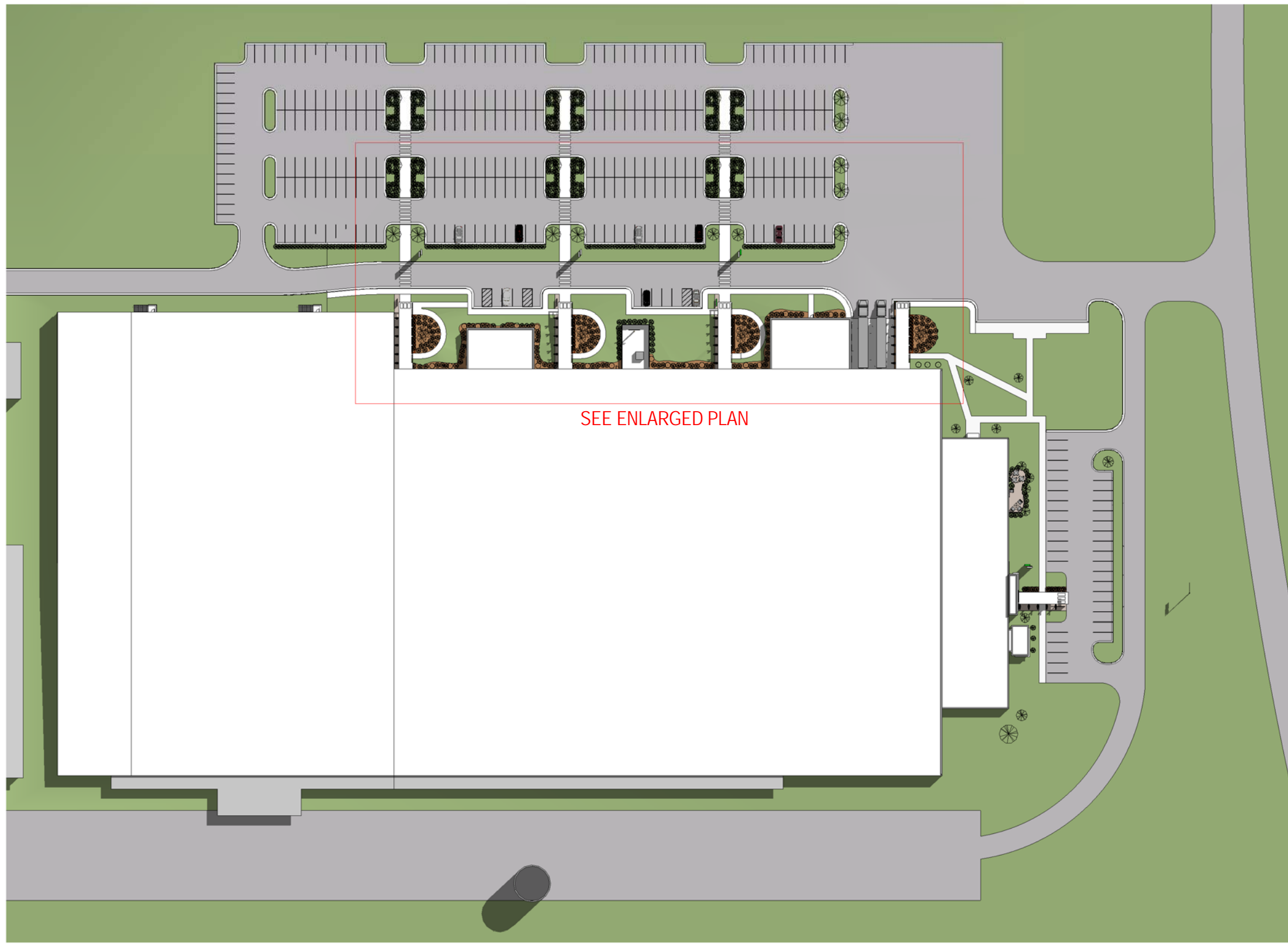
SITE PLAN | 1":100'
